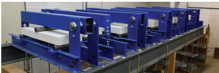
Flexural Creep
